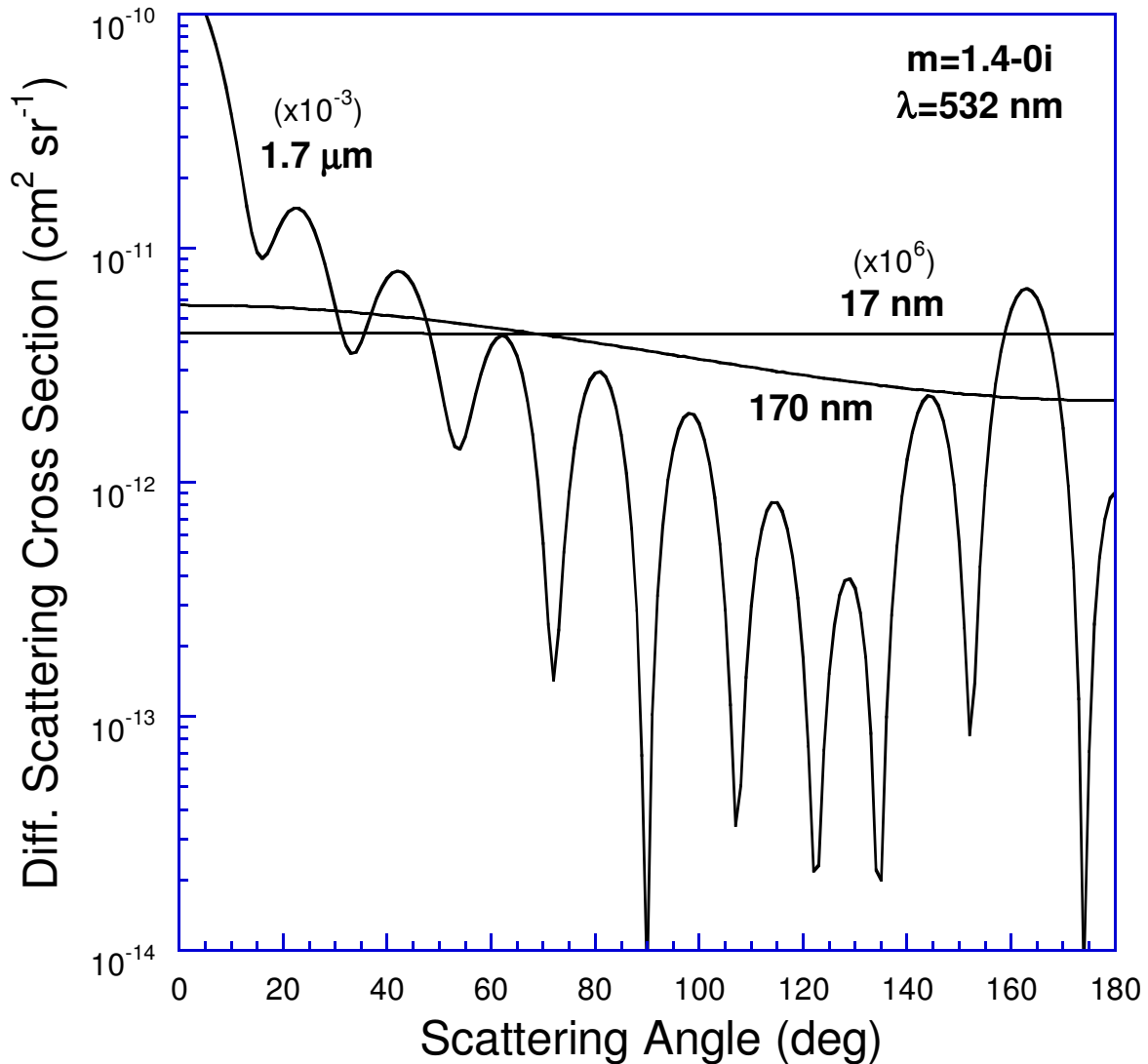
Figure 3. This plot presents the differential scattering cross-section ( \sigma'_{vv} ) as a function of scattering angle \theta (see Figure 2), hence 0^\circ is forward scattering and 180^\circ is backscattering. The smallest particle size of 17 nm ( \alpha = 0.1 ) is well within the Rayleigh regime, and therefore the angular dependence is negligible. The 170 nm particle ( \alpha = 1.0 ) is departing from the Rayleigh regime, and therefore displays some angular variation, with forward scattering beginning to emerge. Note, however, that the function is still monotonic. The 1.7 \mu\text{m} particle ( \alpha = 10 ) is clearly in the Mie regime, where forward scattering dominates. However, note the strong “ripple” structure as a function of scattering angle. This is characteristic of Mie scattering, and is due to the complex interactions of scattered and refracted rays that result in constructive and destructive interference along different paths (i.e. different scattering angles). Note the scale factors in parentheses for the 17 nm and 1.7 \mu\text{m} particle plots, hence these cross-sections vary by more than 10 orders of magnitude for the two-order of magnitude variation in particle size.
