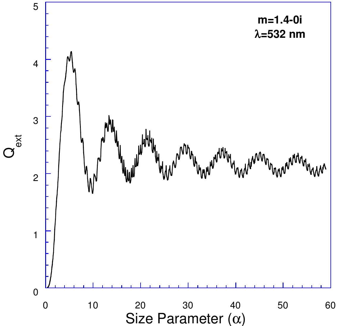
Figure 4. This plot presents the extinction efficiency as a function of size parameter. The extinction efficiency is the extinction cross section ( \sigma_{\text{ext}} ) normalized by the geometric cross section ( \pi a^2 ). For Rayleigh sized particles, the extinction efficiency is much less than 1. For particles in the Mie regime, two characteristics are noted. The ripple or resonance structure observed in the angular scattering plot is also present with extinction, although not as pronounced. In addition, the asymptotic limit of the above plot is 2, meaning that in the large particle limit, twice as much energy is removed as expected based on the geometric cross section. This is contrary to observation, and is referred to as the extinction paradox. In actuality, one half of the energy is removed by scattering/extinction, while the second half is removed via near-forward angle diffraction. Since an observer generally “sees” the diffracted energy, it appears that a large particle only removes energy equal to its actual geometric cross-section.
