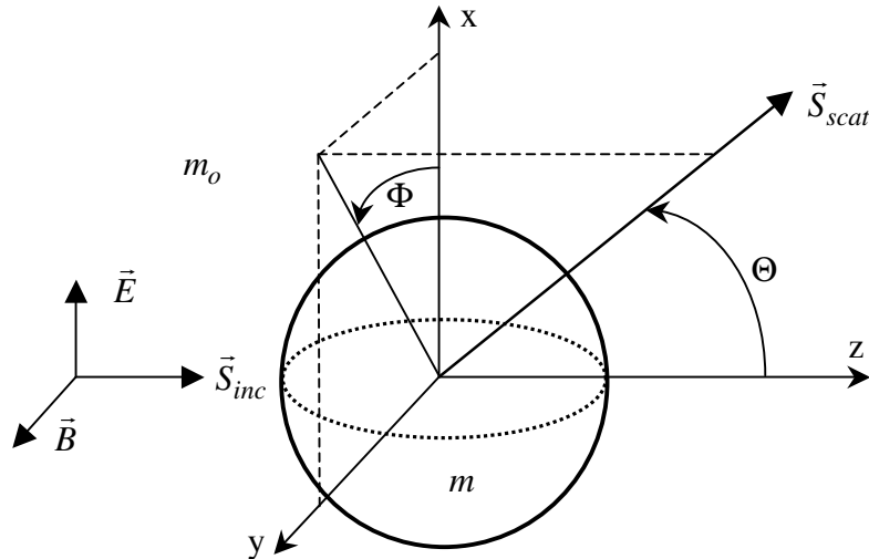
Figure 2. Coordinate geometry for Rayleigh and Mie scattering.
