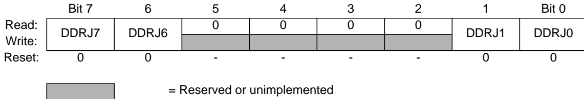
Figure 3-40 Port J Data Direction Register (DDRJ)
