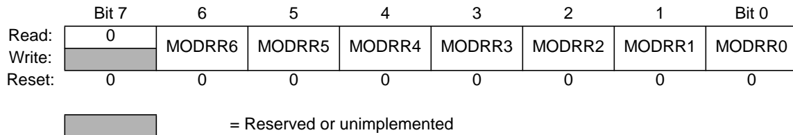
Figure 3-21 Module Routing Register (MODRR)
