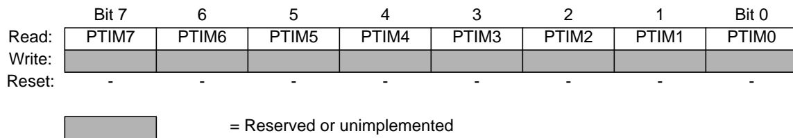
Figure 3-15 Port M Input Register (PTIM)
