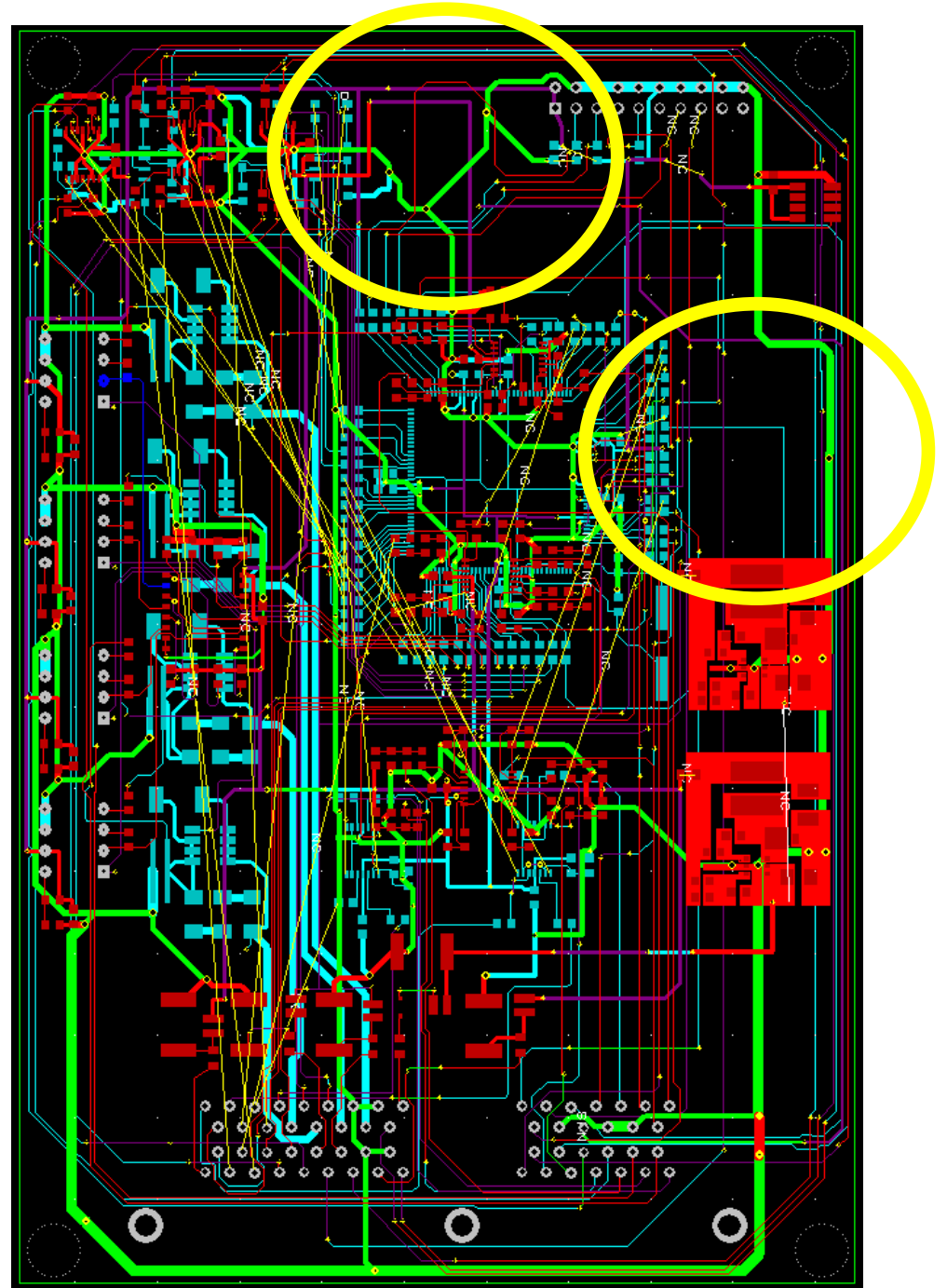
PCB Rev. 5 – Current Design
