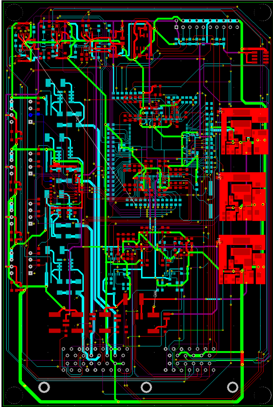
PCB Rev. 2 – Last Year's Design
