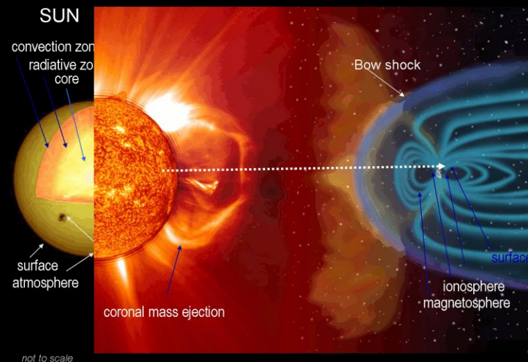
Sun-Earth System: Energy Coupling
