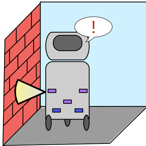
Wall Avoidance
