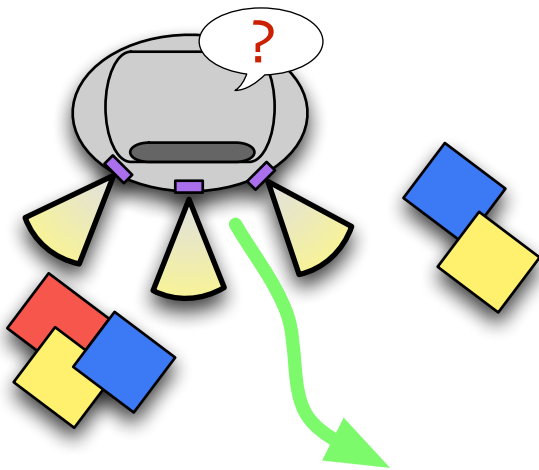
Path Finding
