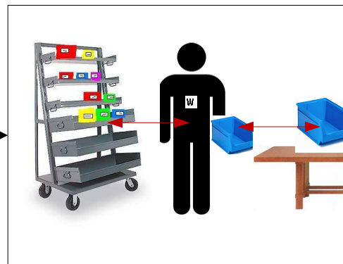
Water spider delivers bins to each station, picks up empty bins.
