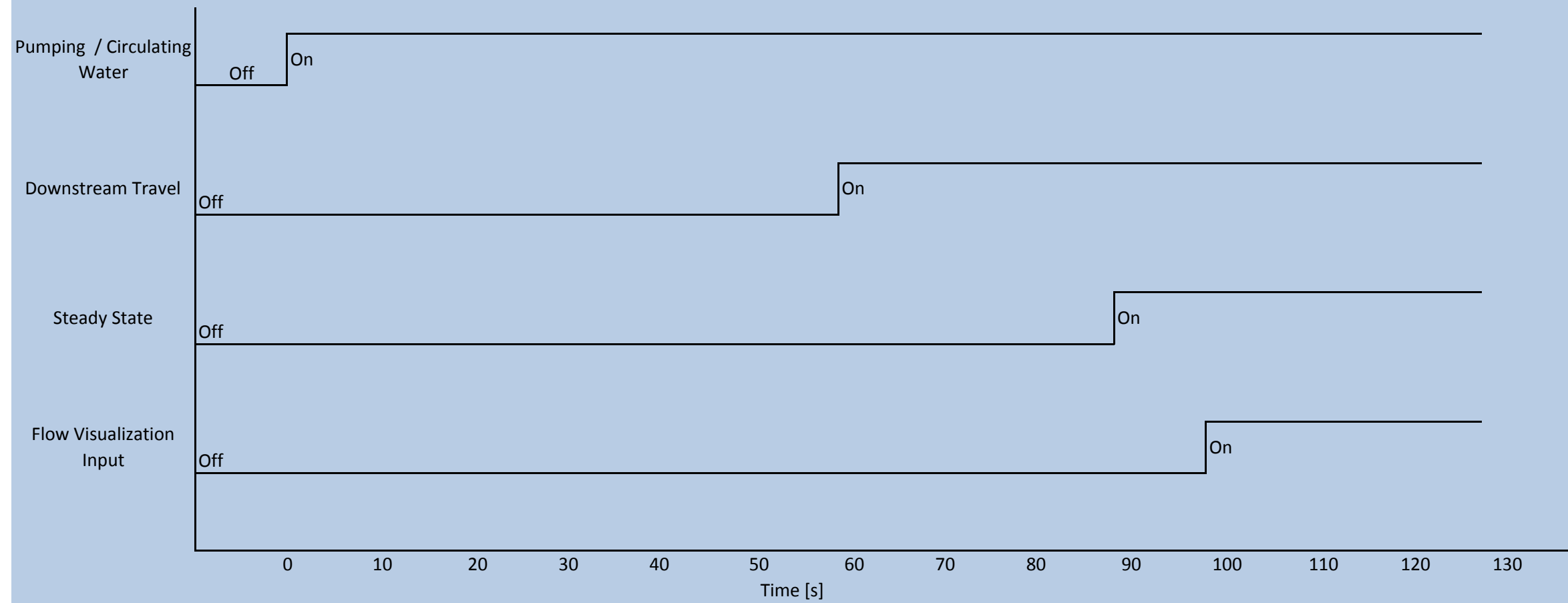
Timing / State Diagram of System
