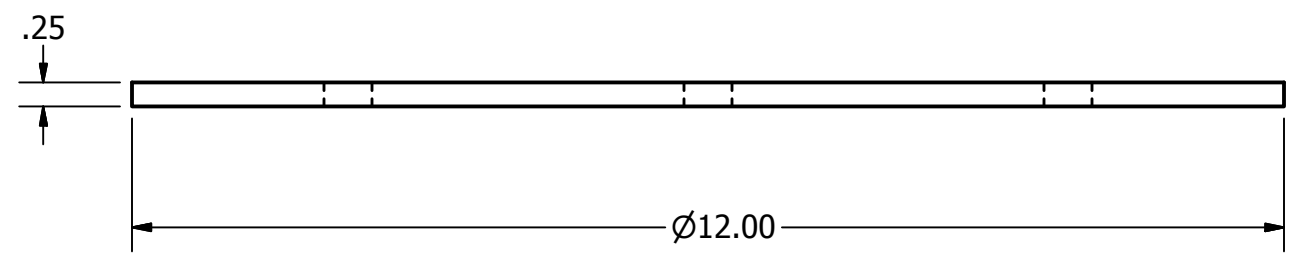
Front View SCALE 1 / 2
