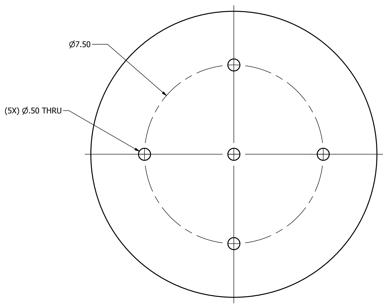
Top View SCALE 1 / 2
