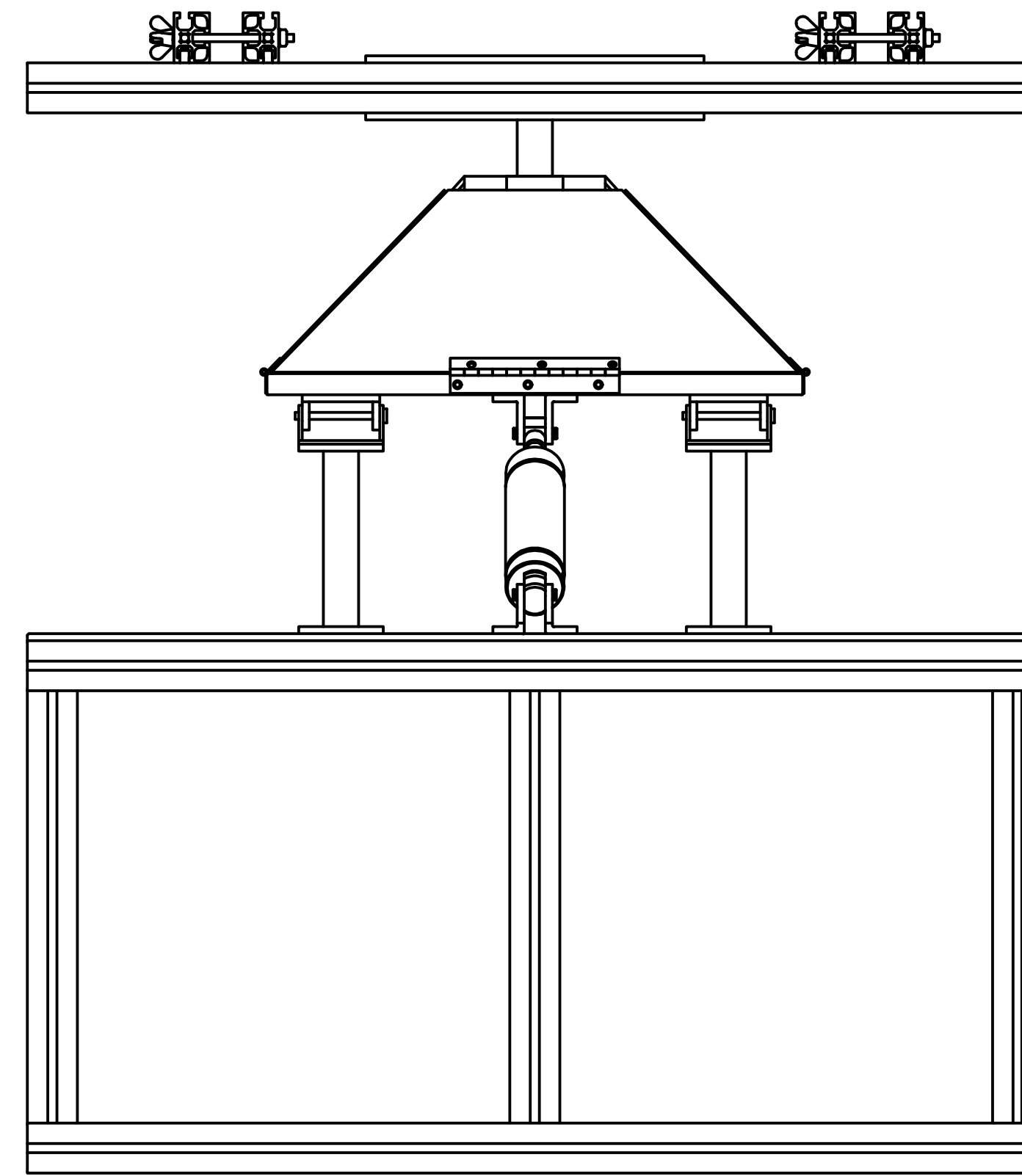
Right View SCALE 1:5
