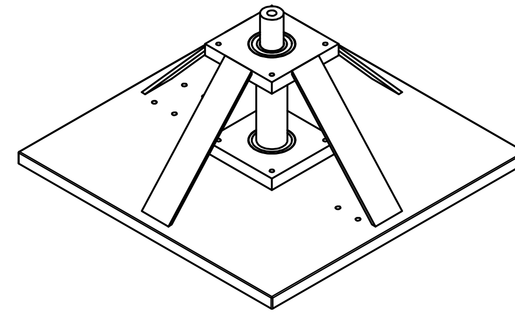
Middle Assembly Interior SCALE 1:5
