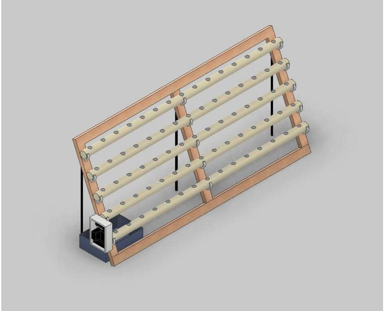
Figure 8. Full-scale CAD layout
