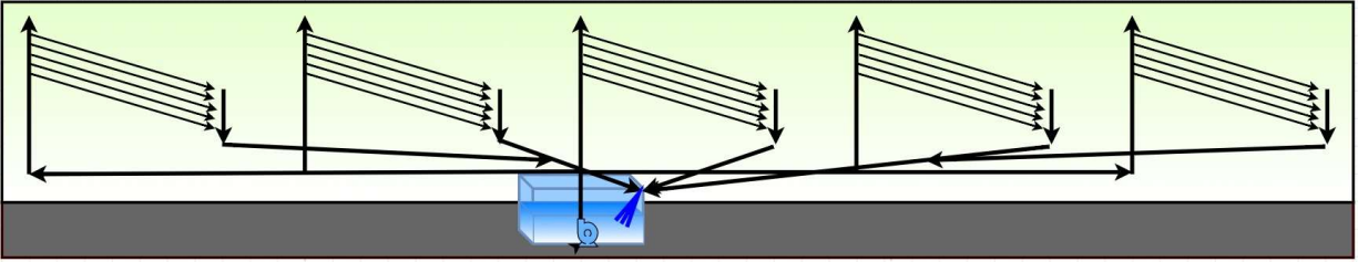
Figure 5. Module Layout (5 units)
