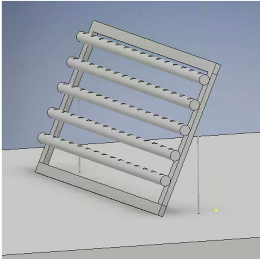
Figure 6. A-Frame CAD layout
