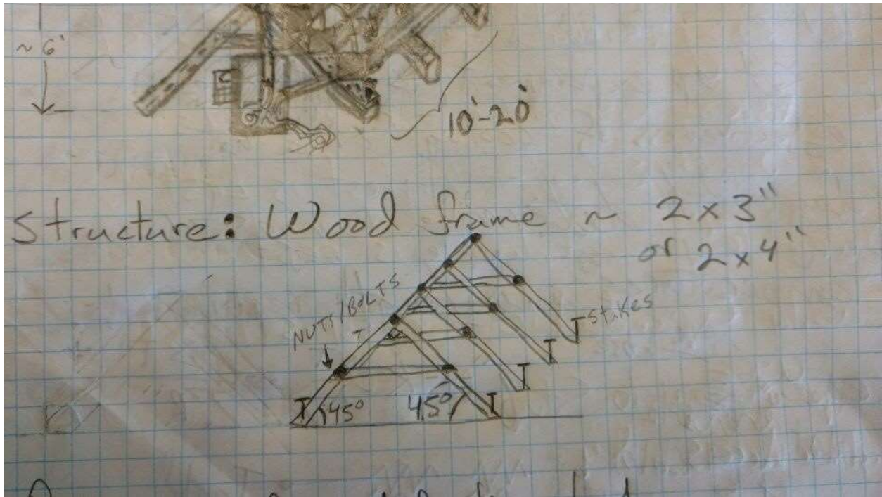
Figure 3. A-Frame design
