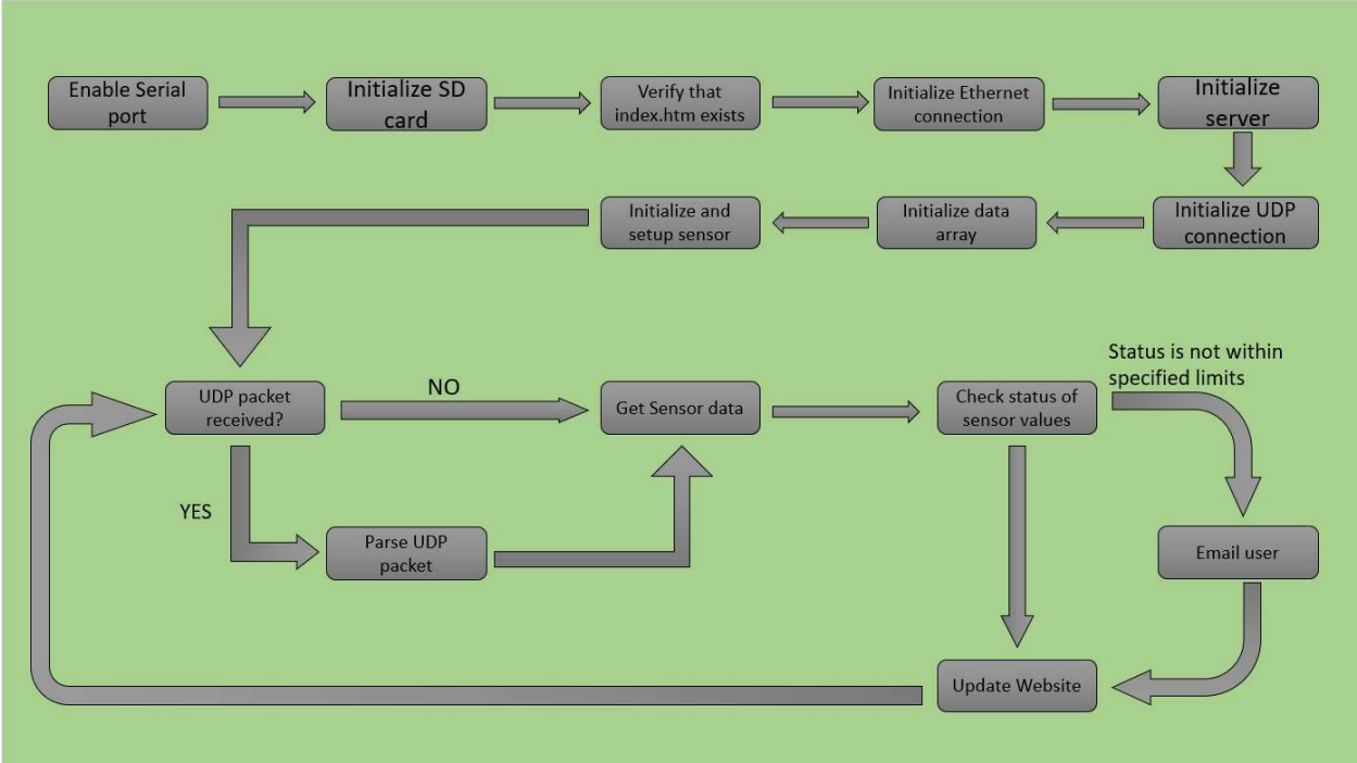
Figure 4.Final Software UML diagram
