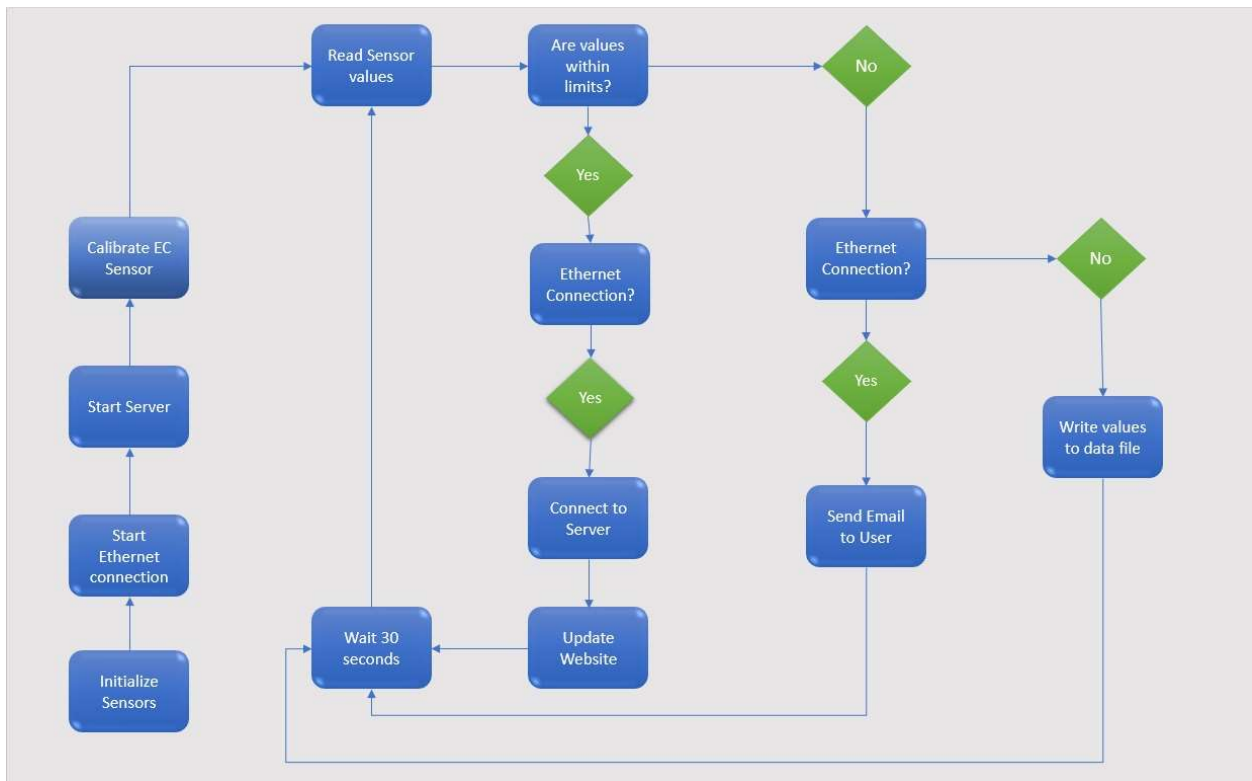
Figure 3. Software UML diagram (detailed design review)
